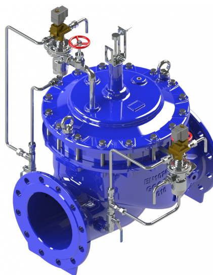
A7MD Pump Control Valve - Mechanical type
